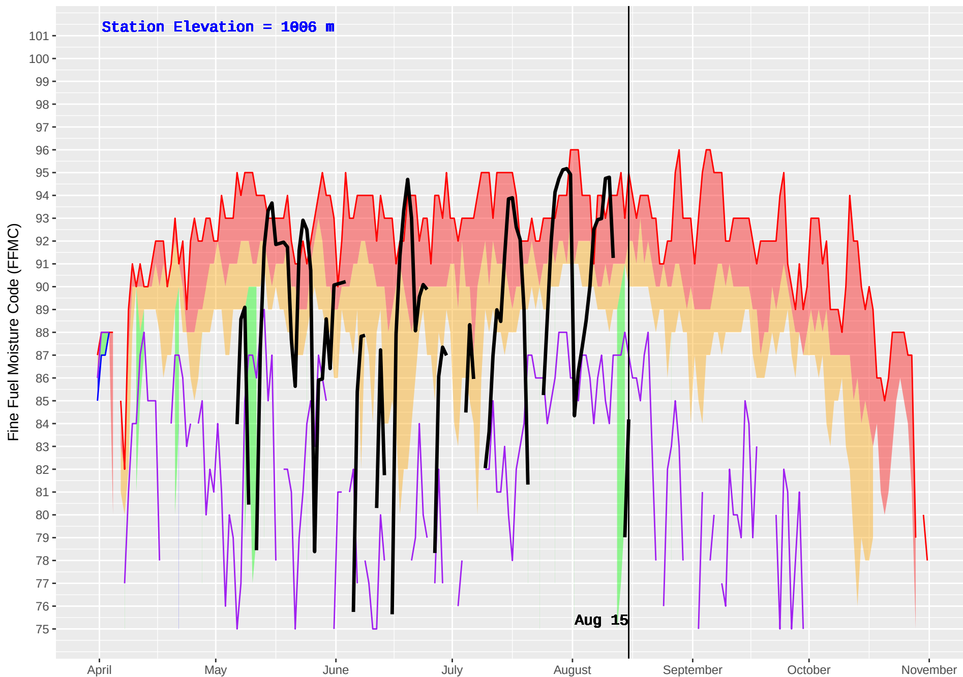
BENSON (228) : Historical (1987–2016) and Current (2018) Daily Fine Fuel Moisture Code (FFMC)
