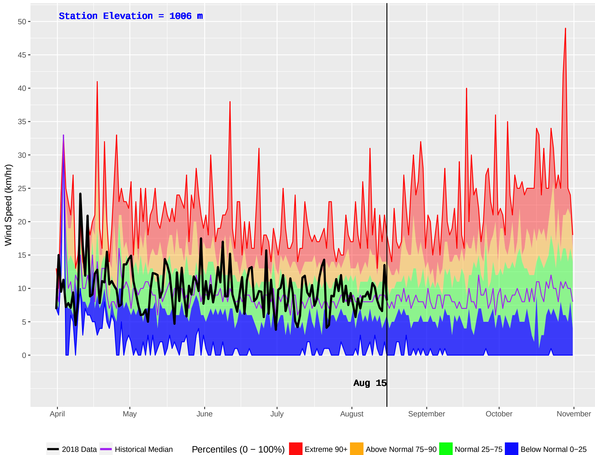
BENSON (228) : Historical (1987–2016) and Current (2018) Daily Wind Speed
