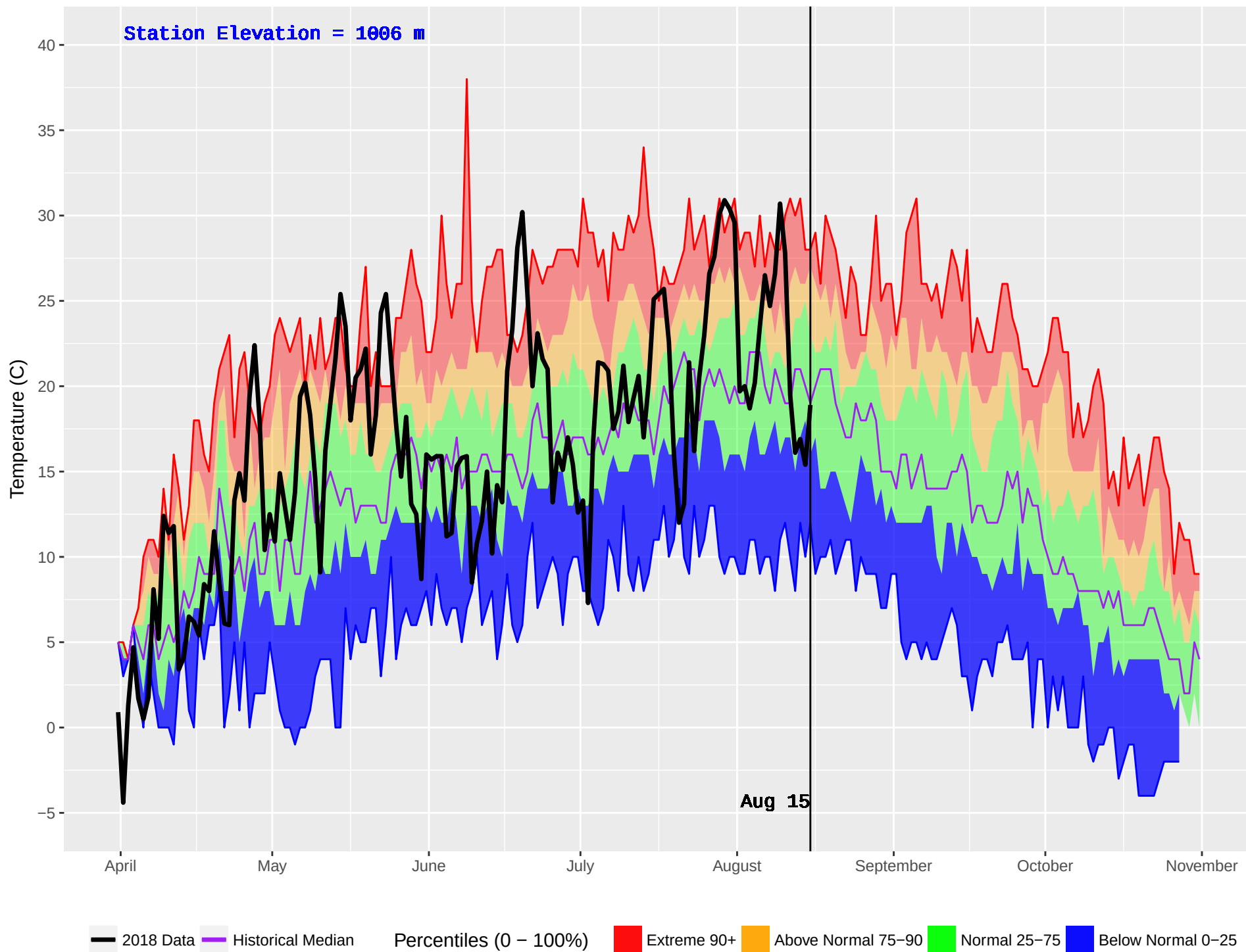
BENSON (228) : Historical (1987–2016) and Current (2018) Daily Temperature
