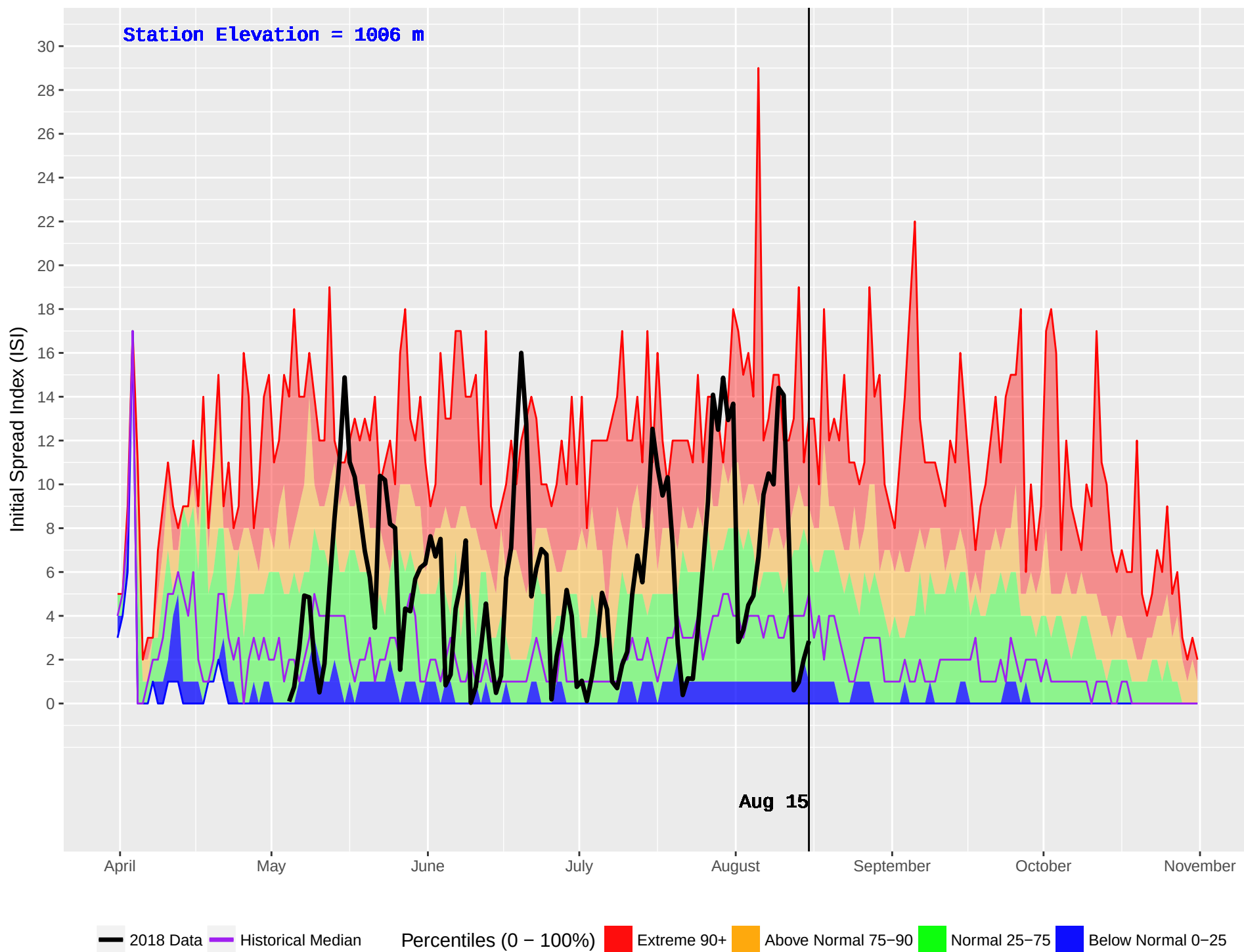
BENSON (228) : Historical (1987–2016) and Current (2018) Daily Initial Spread Index (ISI)
