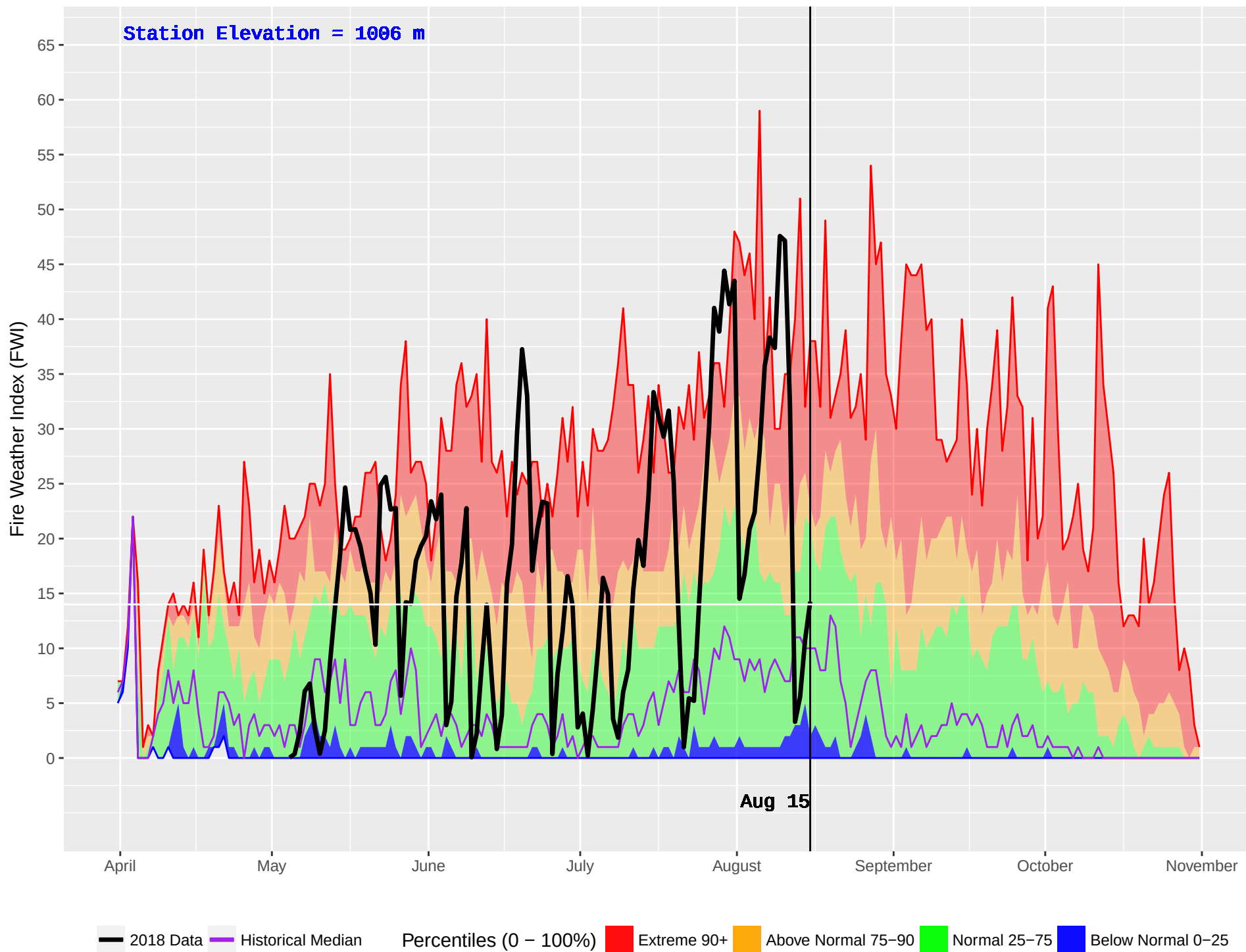
BENSON (228) : Historical (1987–2016) and Current (2018) Daily Fire Weather Index (FWI)
